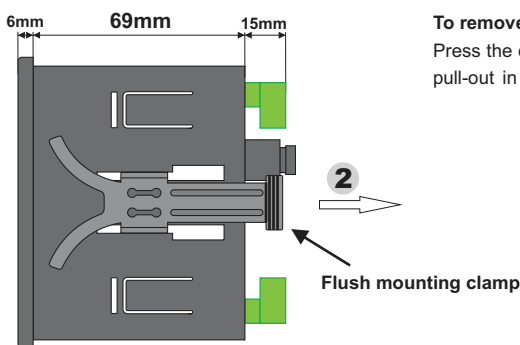
Flush mounting clamp
