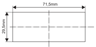
Panel cut-out
